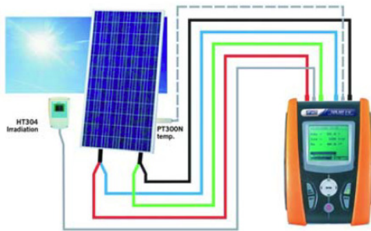
Fig. 3 The measurement of partial shading on solar system
