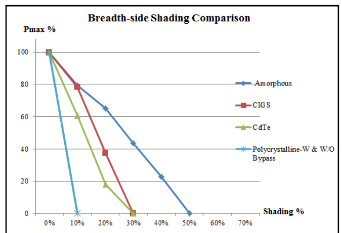
Fig. 9 Comparison of power reduction due to breadth-side shading
